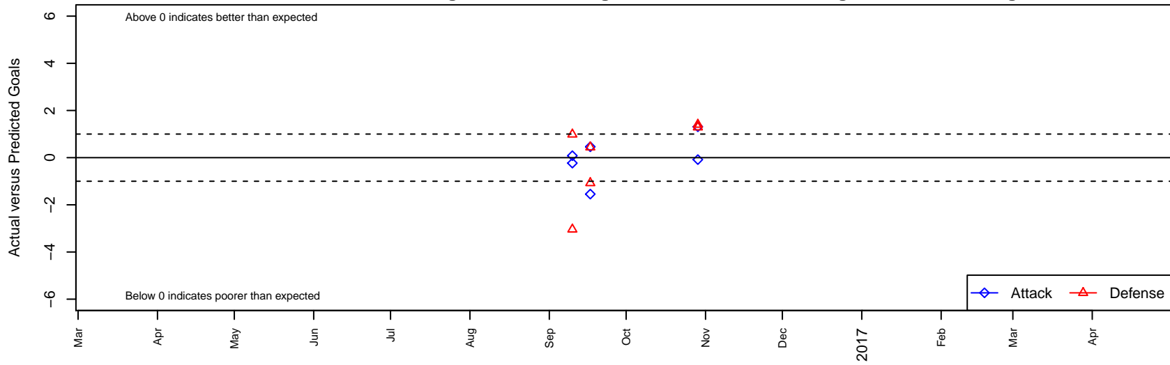
Union County United G03 Dots are actual minus expected GF (blue circles) and GA (red triangles). Blue line is smoothed change in attack strength. Red is smoothed change in defense strength.
